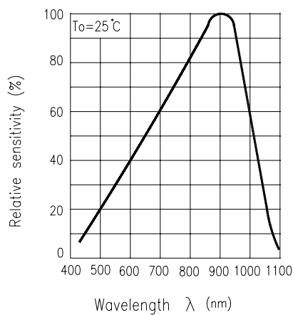
Fig.3 Spectral Sensitivity
