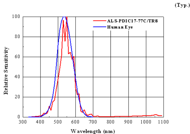
Fig.9 Spectral Response
