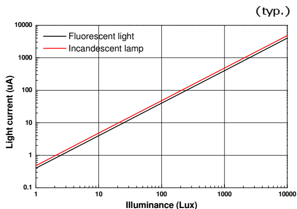
Fig.5 Light Current vs. Illuminance
