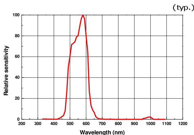
Fig.9 Spectral Response
