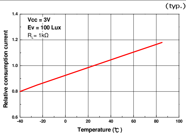
Fig.12 Relative consumption current vs. Temperature
