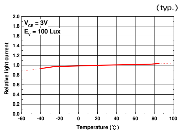
Fig.7 Light current vs. Temperature
