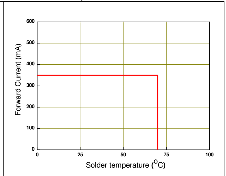
Forward Current Derating Curve, Derating based on T_{j\ MAX} = 125^{\circ}C at torch mode
