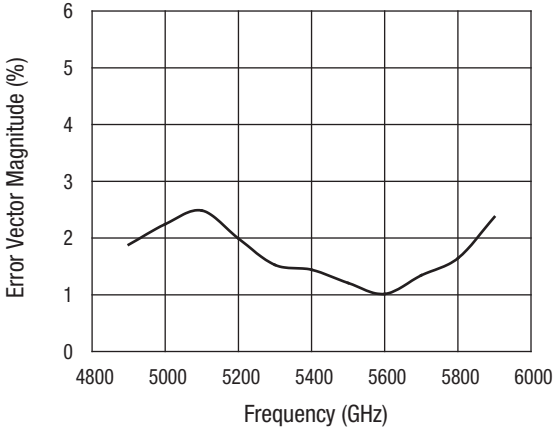
EVM vs. Frequency (P OUT = 15 dBm)
