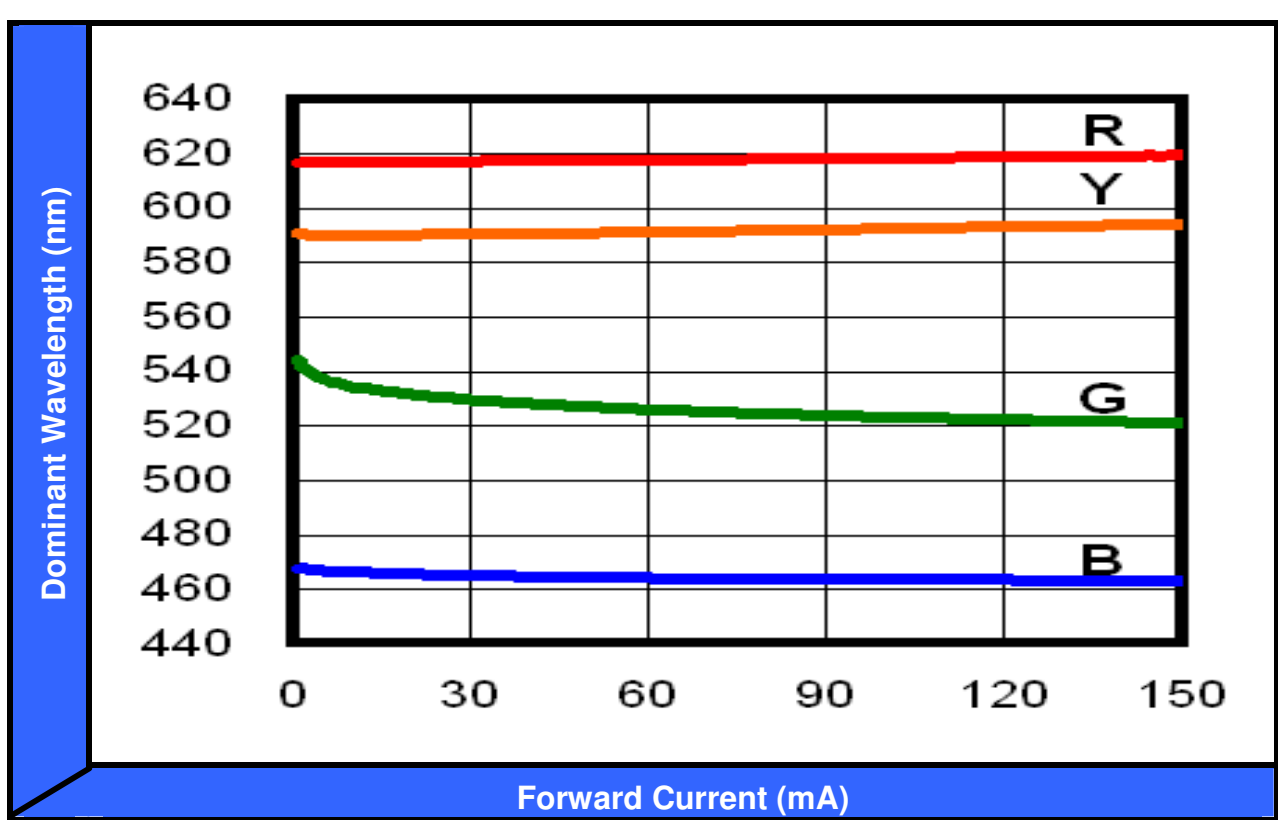
Dominant Wavelength vs. Forward Current (Ta=25 °C)
