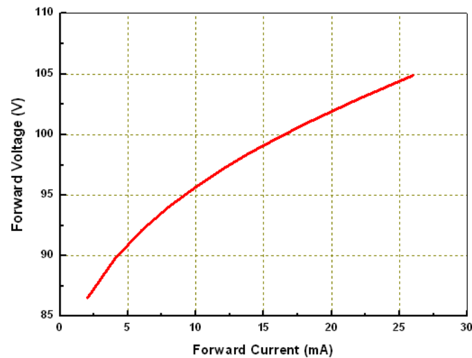
For Warm-White @ Thermal Pad Temperature = 25°C
