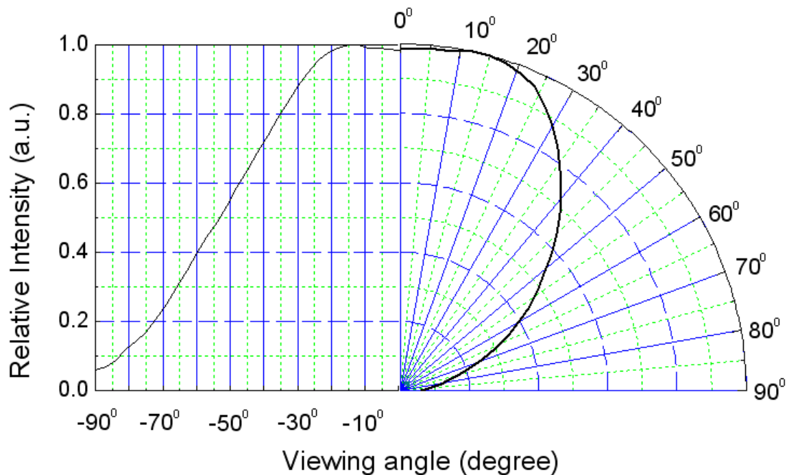
Typical Spatial Radiation Pattern for Warm-White
