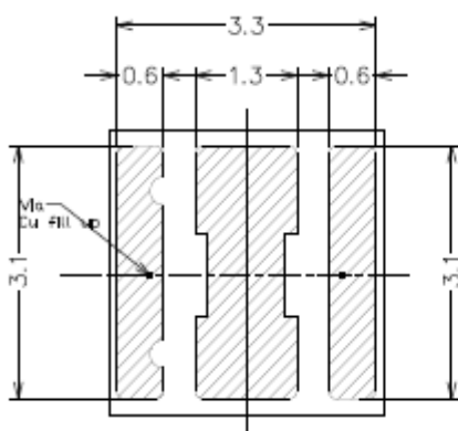
Solder pad design
