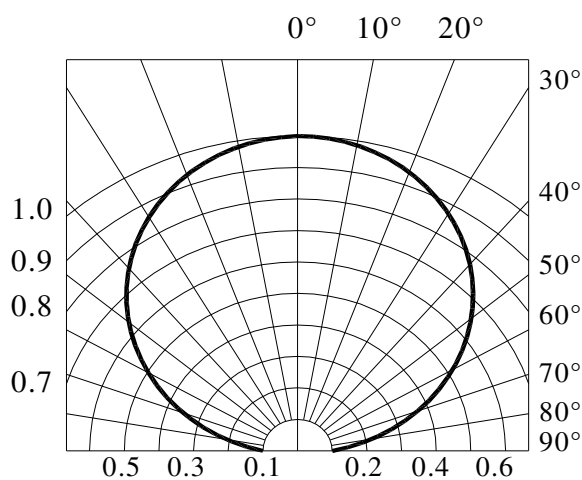
Fig.6 - Radiation Diagram
