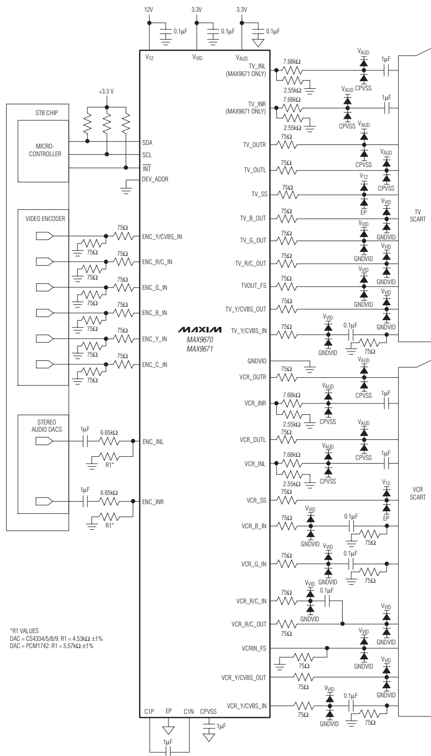
Figure 18. Application Circuit to Connect Series Resistors and External ESD Protection Diodes at MAX9670/MAX9671 Outputs
