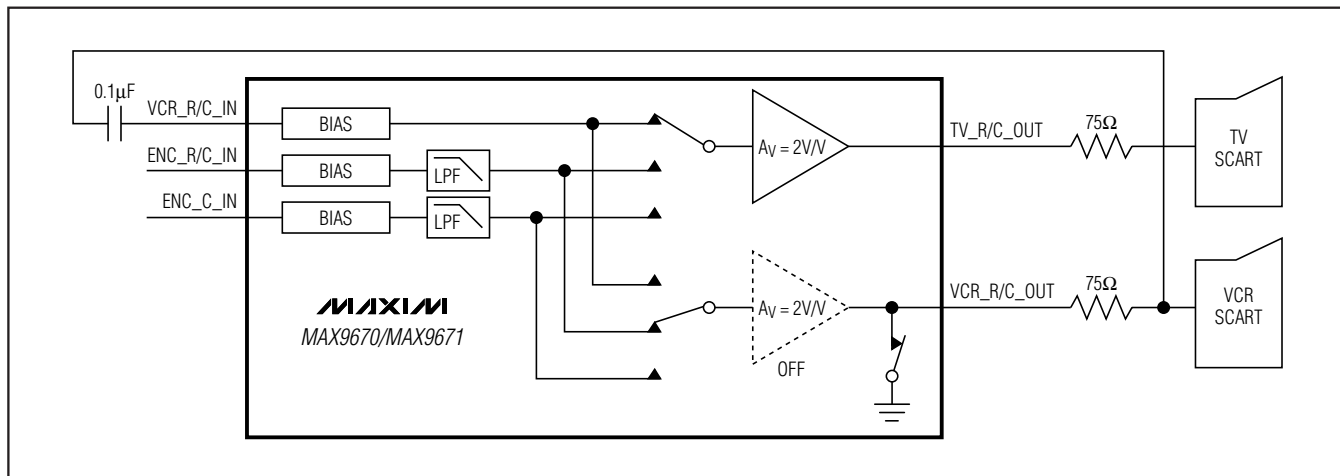
Figure 16. VCR_R/C_IN receives chroma signal from VCR SCART connector. Notice that the pulldown switch on VCR_R/C_OUT is closed and that the gain-of-2 amplifier is off. The chroma signal from VCR SCART is looped through to the TV SCART in the above configuration.
