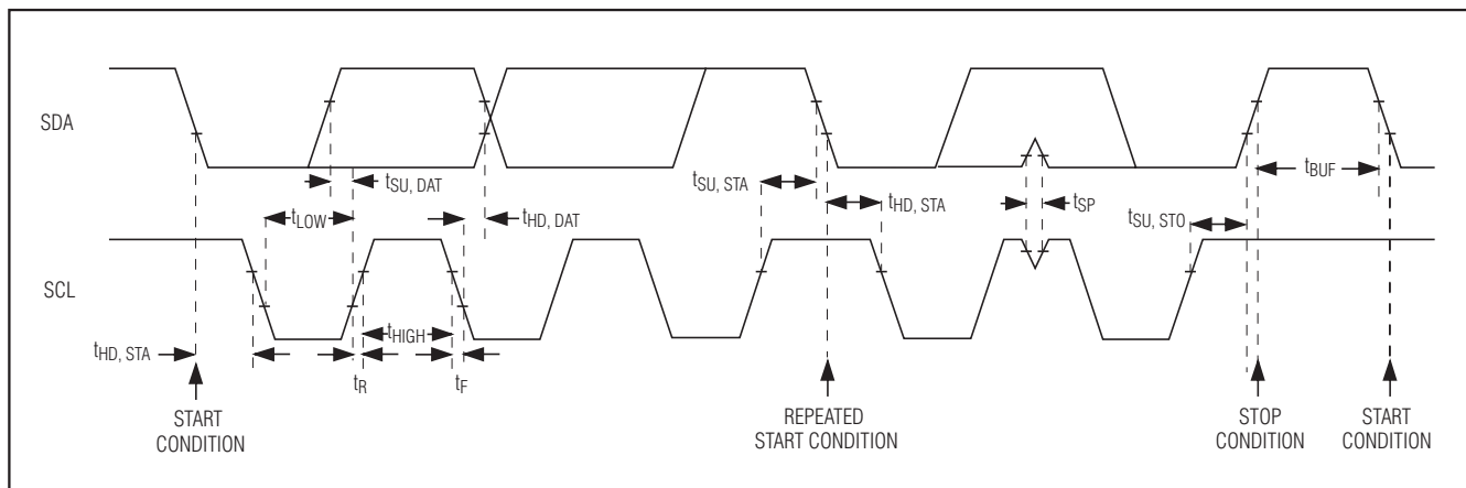
Figure 6. I 2 C Serial-Interface Timing Diagram
