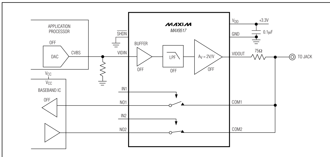
Figure 5. Digital Output Configuration
