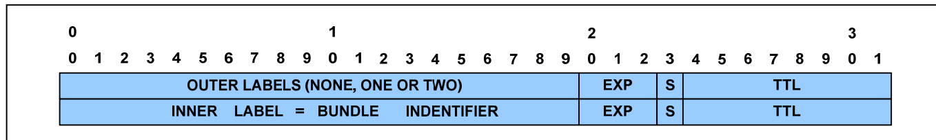
Figure 10-15. MPLS Header Format
