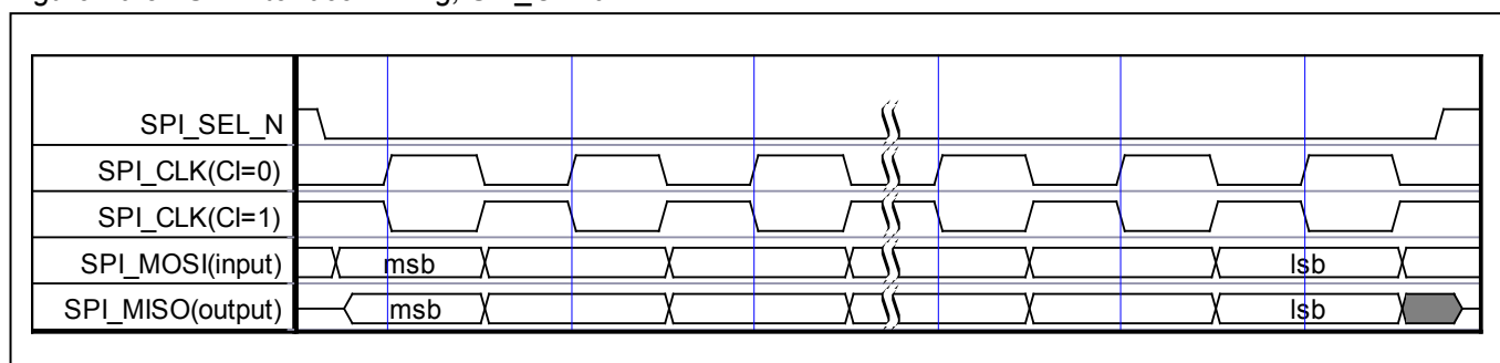
Figure 10-8. SPI Interface Timing, SPI_CP=0
