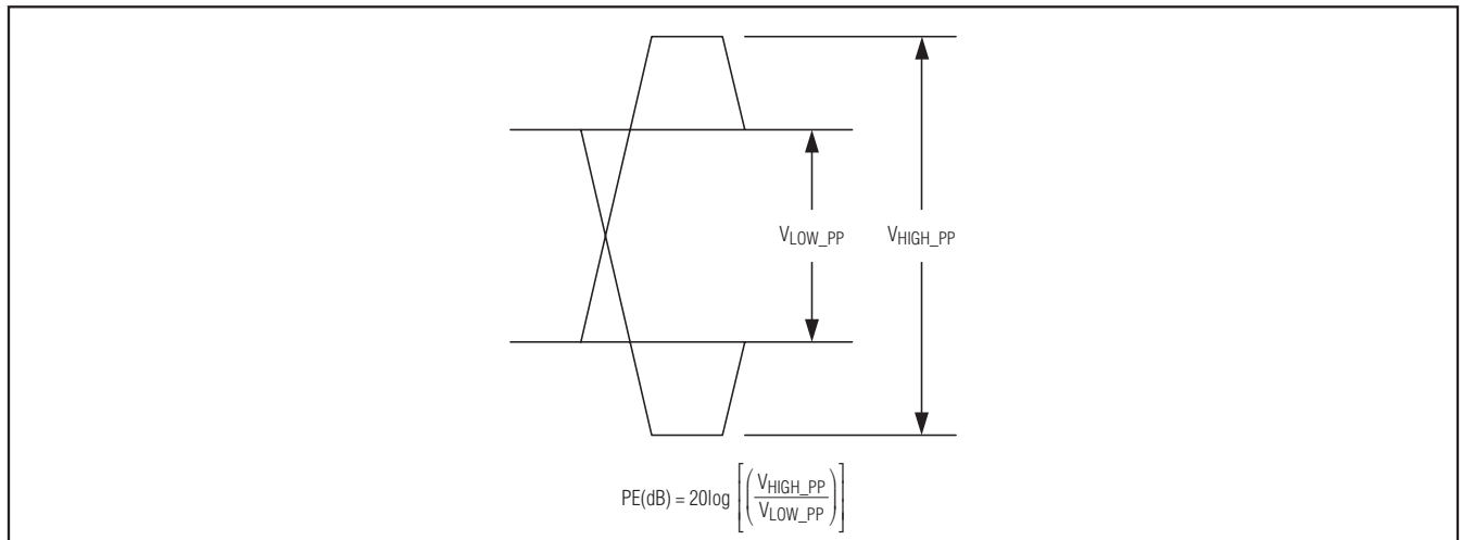
Figure 1. Output Preemphasis
