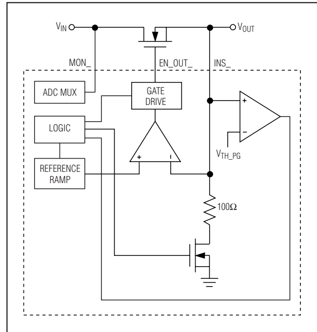
Figure 5. Closed-Loop Tracking
