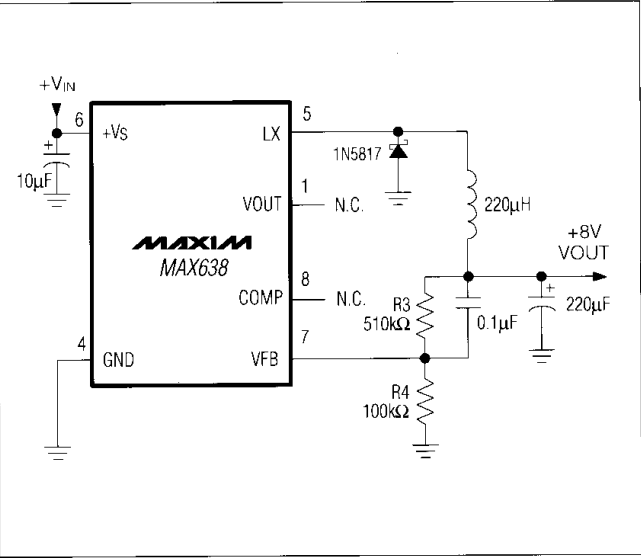
Figure 4. Adjustable Output Operation
