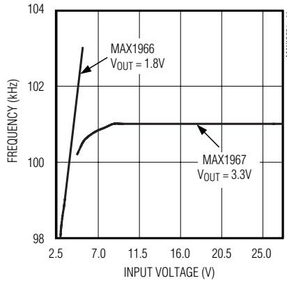
FREQUENCY vs. INPUT VOLTAGE
