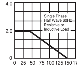
FIG. 2 - TYPICAL FORWARD CURRENT DERATING CURVE
