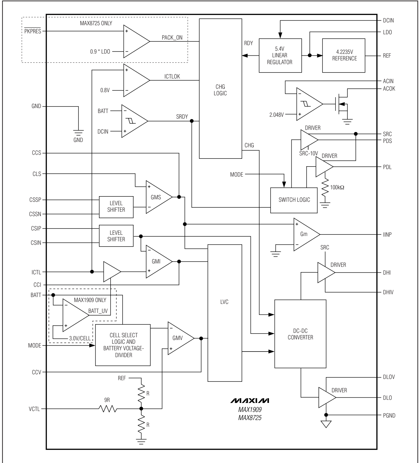
Figure 3. Functional Diagram
