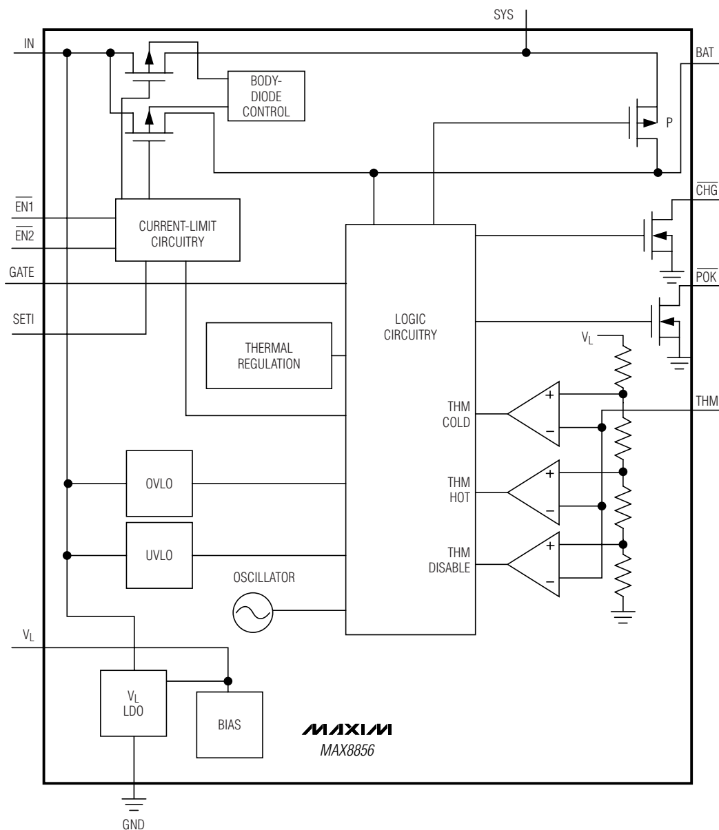
Figure 2. MAX8856 Block Diagram
