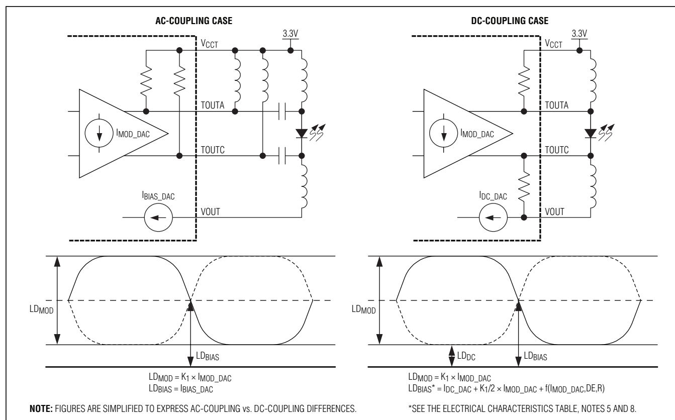
Figure 3. AC-/DC-Coupling Cases
