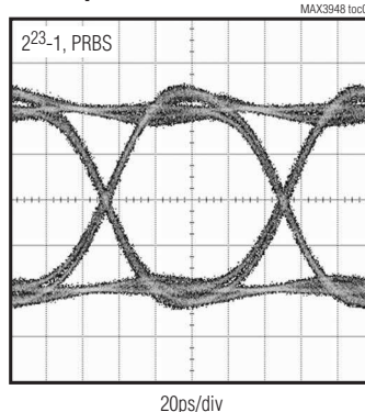
10.3Gbps ELECTRICAL EYE DIAGRAM
