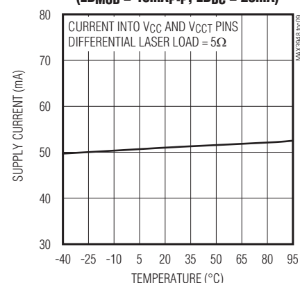
SUPPLY CURRENT vs. TEMPERATURE (LD MOD = 40mA P-P , LD DC = 20mA)
