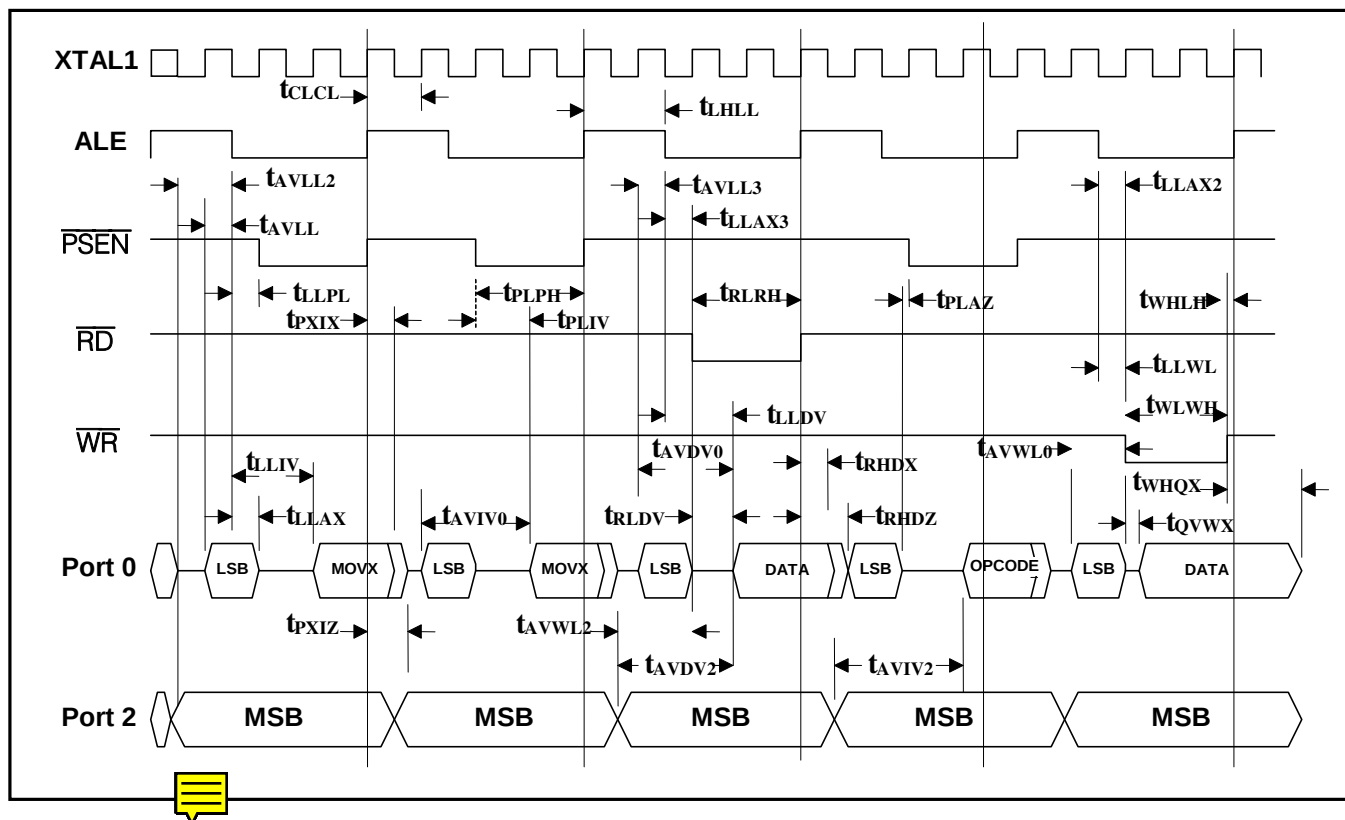
Figure 1. Nonpage Mode Timing
