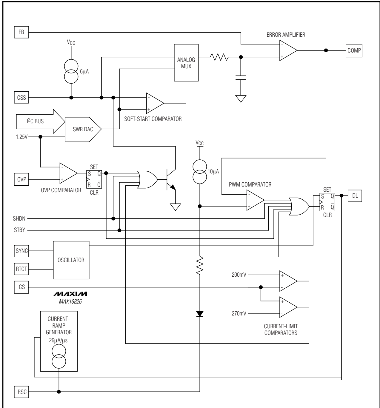
Figure 2. Switch Regulator Controller Block Diagram
