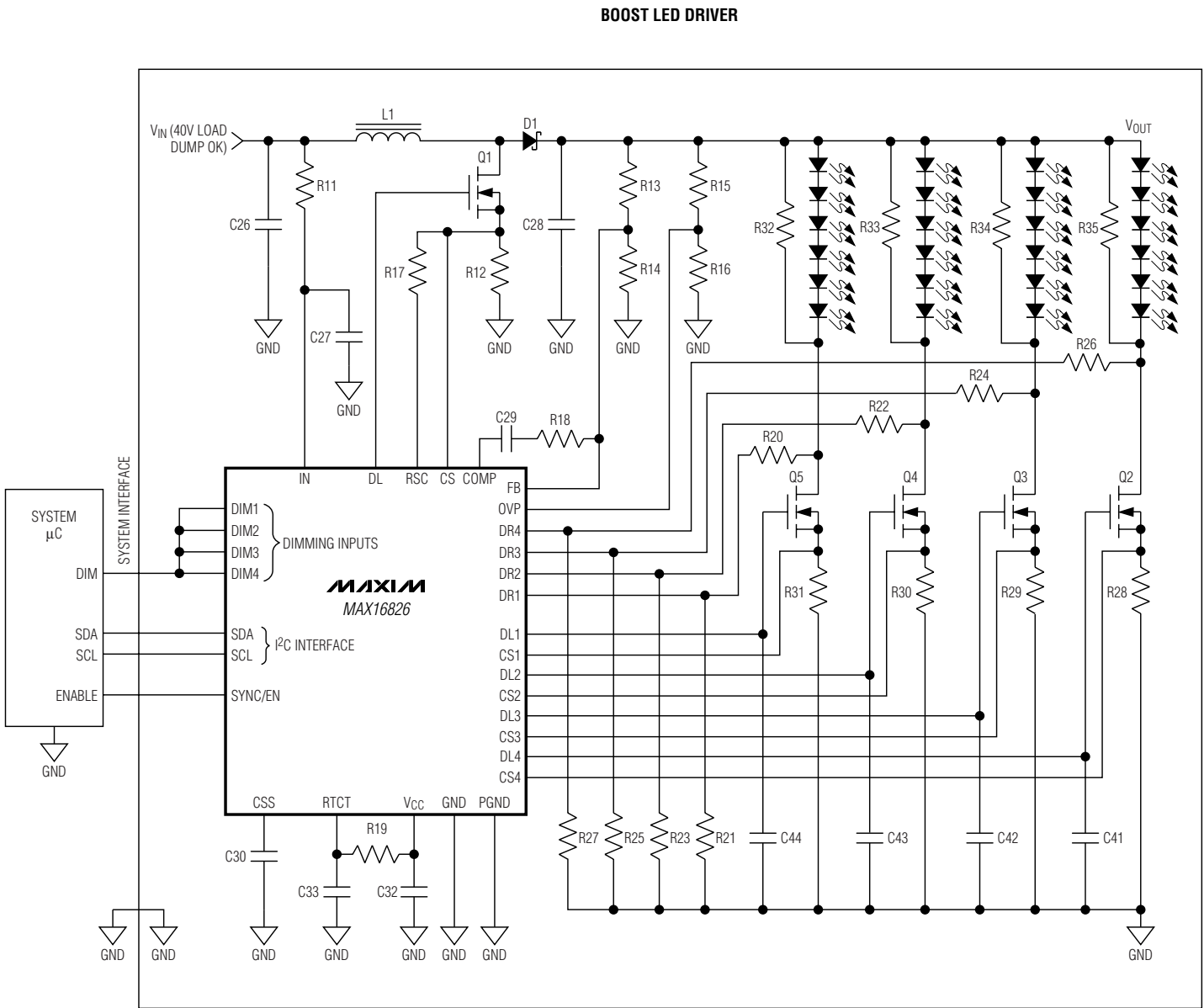
Typical Application Circuit
