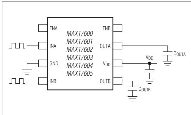
Figure 4. Test Circuit for the Timing Diagrams
