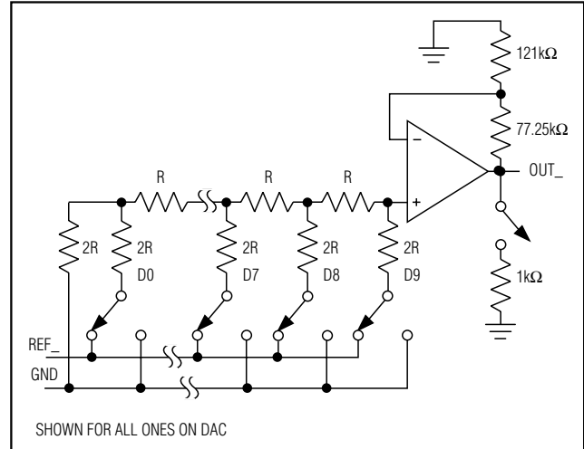
Figure 3. Simplified DAC Circuit Diagram
