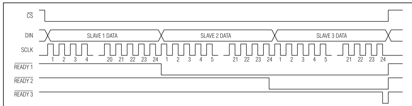
Figure 4. \overline{READY} Timing
