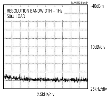
DC NOISE SPECTRUM, FFT PLOT BUFFERED OUTPUT
