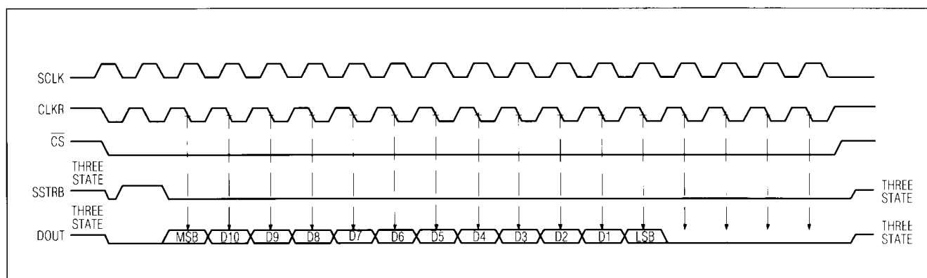
Figure 16. MAX190/MAX191 TMS320C4x Interface Timing
