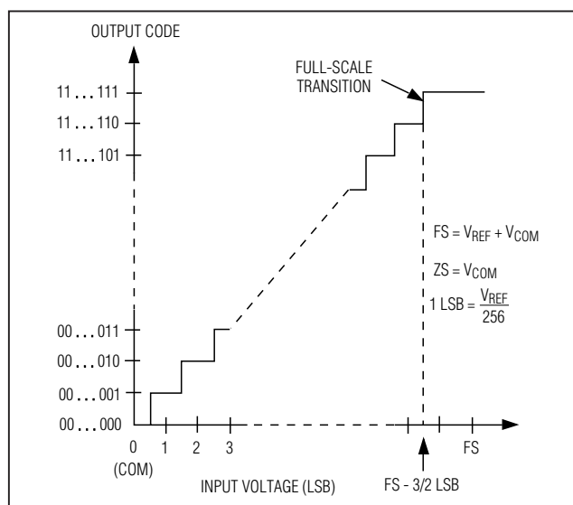
Figure 8. Unipolar Transfer Function, Full Scale (FS) = V_{\text{REF}}
