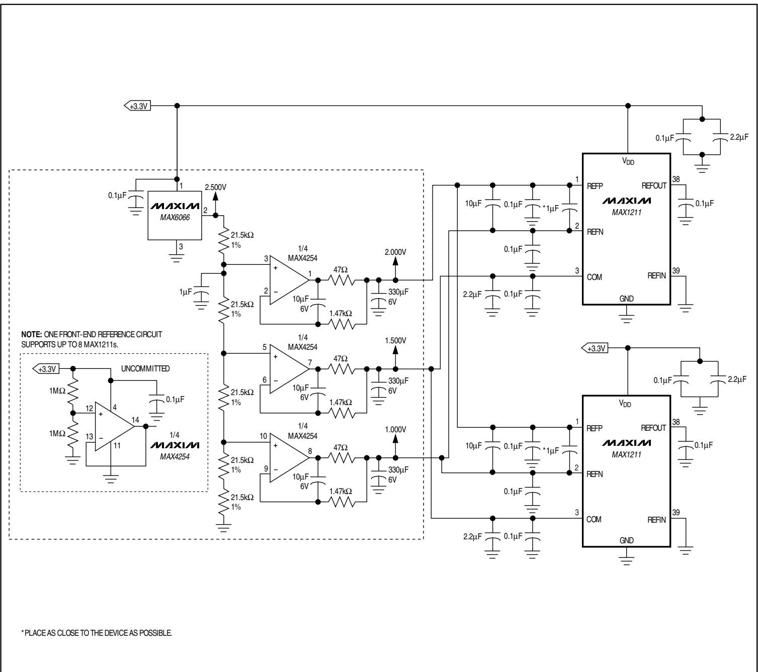
Figure 13. External Unbuffered Reference Driving Eight ADCs with MAX4254 and MAX6066
