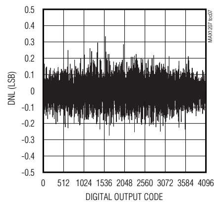
DIFFERENTIAL NONLINEARITY
