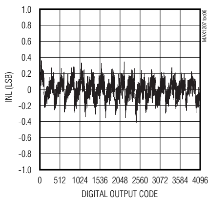
INTEGRAL NONLINEARITY
