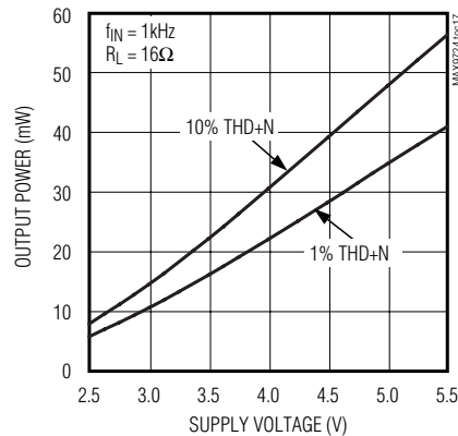
OUTPUT POWER vs. SUPPLY VOLTAGE (TQFN)
