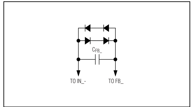
Figure 16. Connection of Output Limiting Diodes
