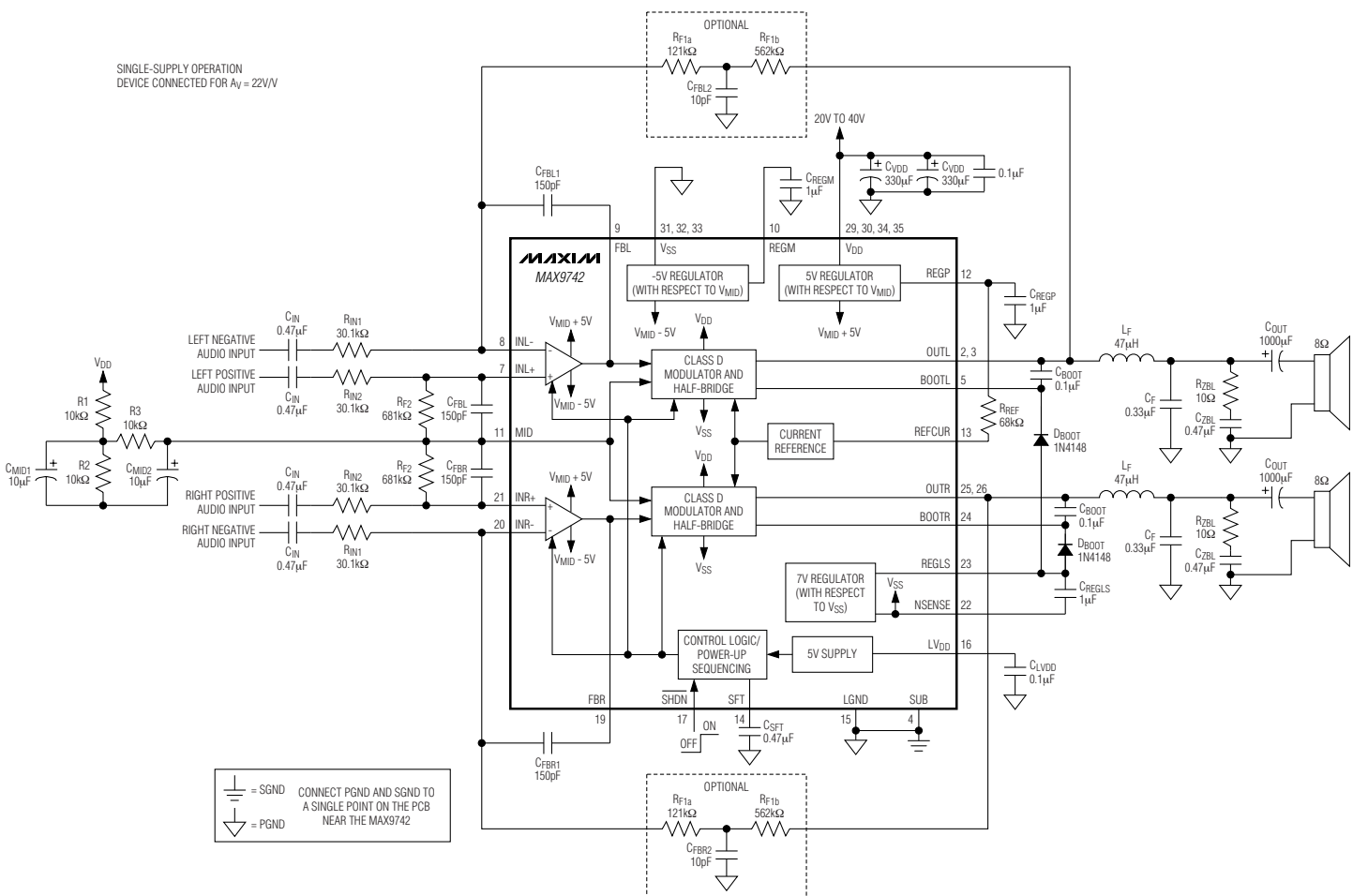
Typical Application Circuits/Functional Diagrams
