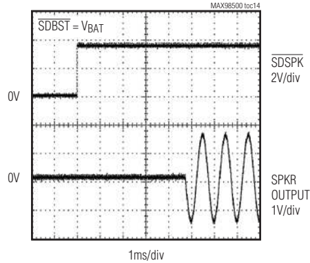
TURN-ON RESPONSE
