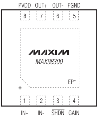
TDFN (2mm x 2mm)
