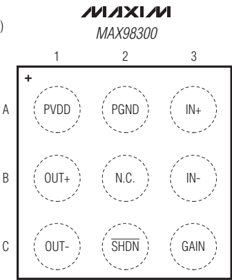
WLP (1.2mm x 1.2mm, 0.4mm pitch)
