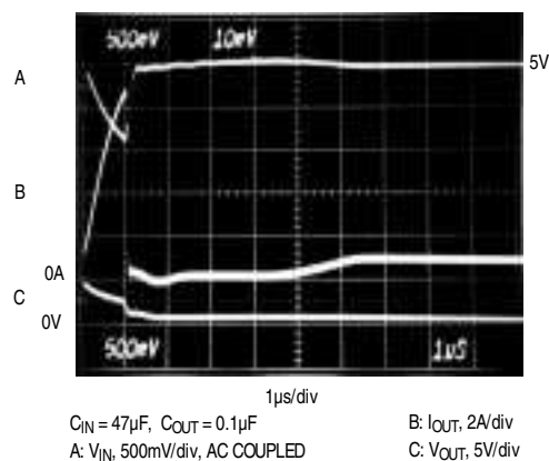
CURRENT-LIMIT RESPONSE (MAX891L, R_L = 0.5\Omega )
