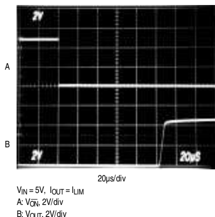
SWITCH TURN-ON TIME
