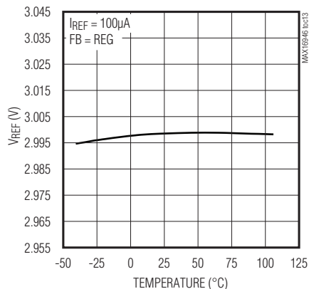
REF OUTPUT VOLTAGE vs. TEMPERATURE
