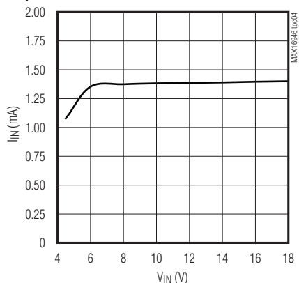
OPERATING SUPPLY CURRENT vs. SUPPLY VOLTAGE (MAX16946/MAX16947 SWITCH CONFIGURATION)
