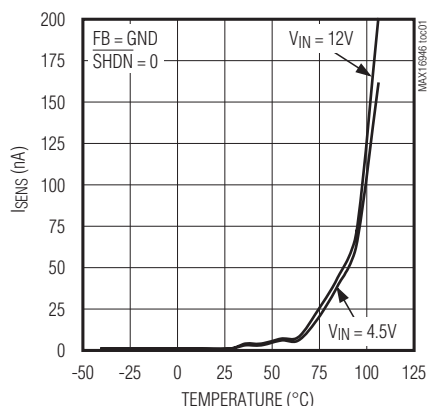
SENSE LEAKAGE CURRENT vs. TEMPERATURE
