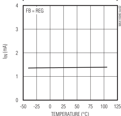
OPERATING SUPPLY CURRENT vs. TEMPERATURE (MAX16946 8.5V LDO CONFIGURATION)
