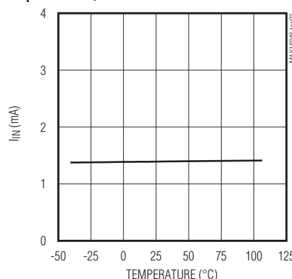
OPERATING SUPPLY CURRENT vs. TEMPERATURE (MAX16946/MAX16947 SWITCH CONFIGURATION)
