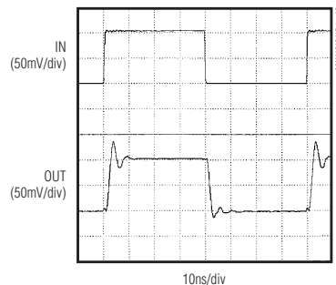
MAX4313 SMALL-SIGNAL PULSE RESPONSE ( C_L = 22pF )
