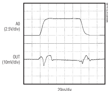
CHANNEL-SWITCHING TRANSIENT
