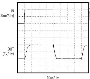
MAX4313 LARGE-SIGNAL PULSE RESPONSE
