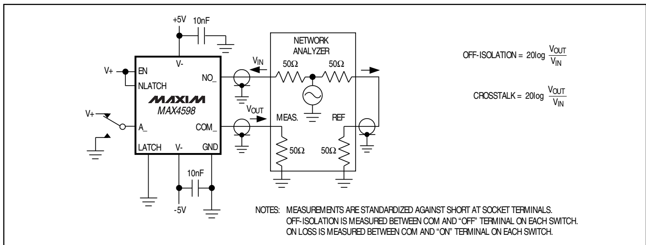
Figure 5. Off-Isolation/Crosstalk
