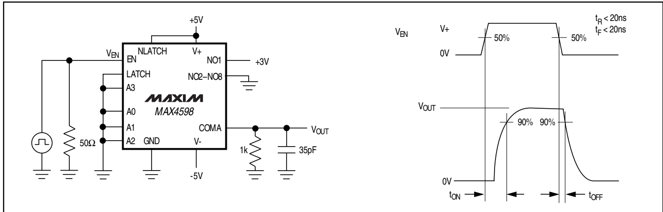
Figure 3. Enable Switching Time
