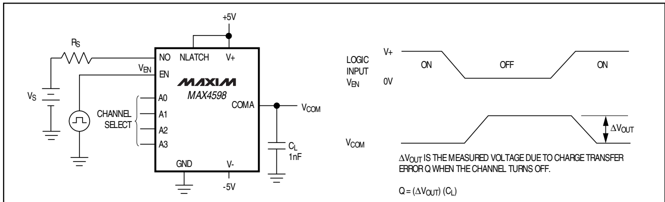
Figure 4. Charge Injection
