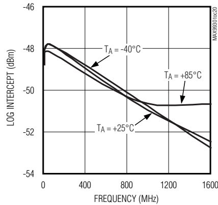
MAX9931 LOG INTERCEPT vs. FREQUENCY
