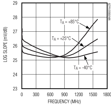
LOG SLOPE vs. FREQUENCY
