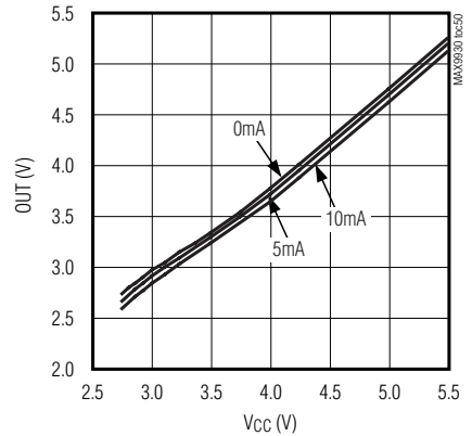
MAXIMUM OUTPUT VOLTAGE vs. V_{CC} BY LOAD CURRENT
