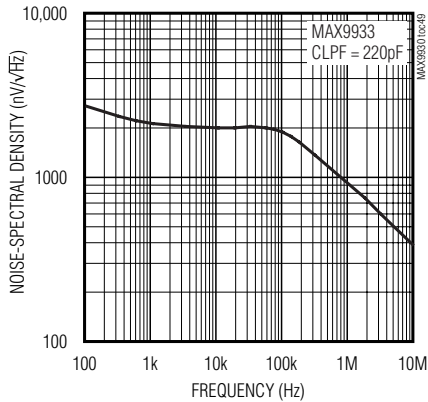
MAIN OUTPUT NOISE-SPECTRAL DENSITY
