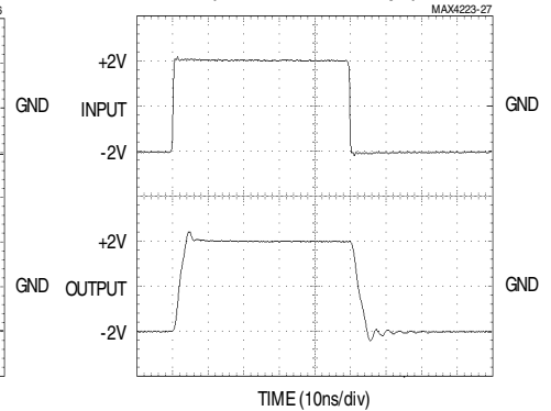
MAX4223/MAX4225/MAX4226 LARGE-SIGNAL PULSE RESPONSE ( A_{vCL} = +1 , C_L = 25pF )
