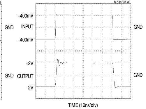
MAX4224/MAX4227/MAX4228 LARGE-SIGNAL PULSE RESPONSE ( A_{vCL} = +5 )
