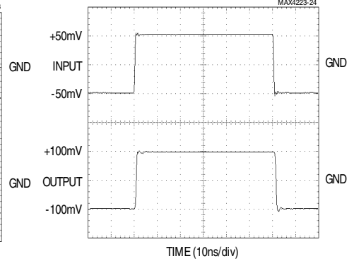
MAX4224/MAX4227/MAX4228 SMALL-SIGNAL PULSE RESPONSE ( A_{vCL} = +2 )
