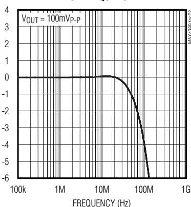
SMALL-SIGNAL GAIN vs. FREQUENCY
