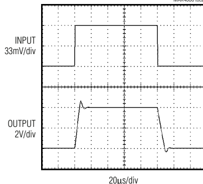
MAX4081S LARGE-SIGNAL TRANSIENT RESPONSE MAX4080 toc27
