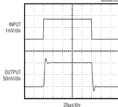
MAX4081S SMALL-SIGNAL TRANSIENT RESPONSE MAX4080 toc21
