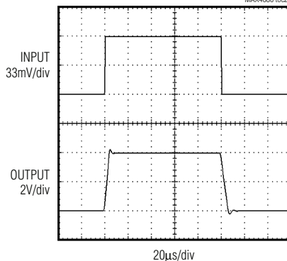
MAX4080S LARGE-SIGNAL TRANSIENT RESPONSE MAX4080 toc24
