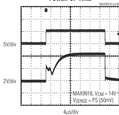
POWER-UP TIME
