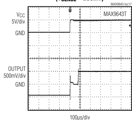
STARTUP DELAY (VSENSE = 200mV)
