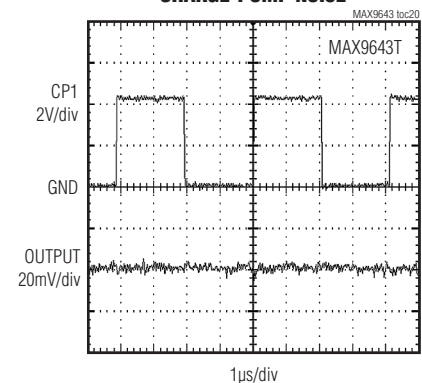
CHARGE-PUMP NOISE
