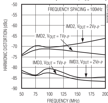
INTERMODULATION DISTORTION vs. FREQUENCY (MAX9627, V_{CC} = 3.3V )
