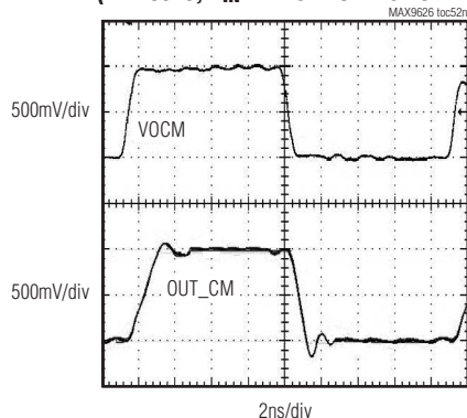
VOCM TRANSIENT RESPONSE (MAX9626, V_{IN} = 1.15V TO 2.15V STEP)
