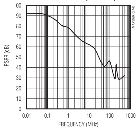
POWER-SUPPLY REJECTION RATIO vs. FREQUENCY (MAX9628)
