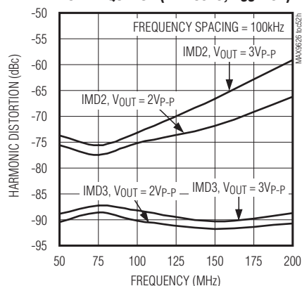
INTERMODULATION DISTORTION vs. FREQUENCY (MAX9628, V_{CC} = 5V )
