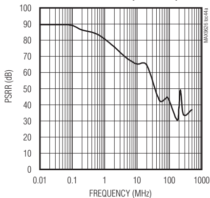
POWER-SUPPLY REJECTION RATIO vs. FREQUENCY (MAX9627)
