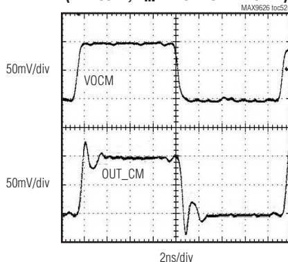
VOCM TRANSIENT RESPONSE (MAX9627, V_{IN} = 1.6V TO 1.7V STEP)
