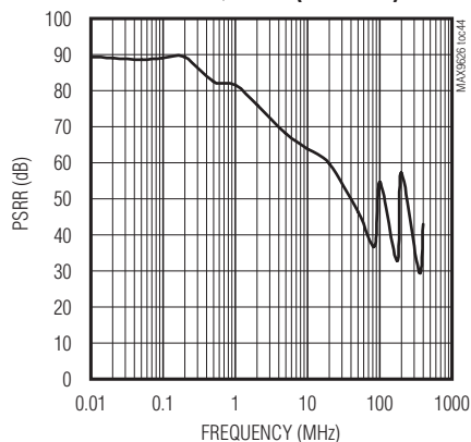
POWER-SUPPLY REJECTION RATIO vs. FREQUENCY (MAX9626)
