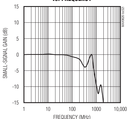
VOCM SMALL-SIGNAL GAIN vs. FREQUENCY
