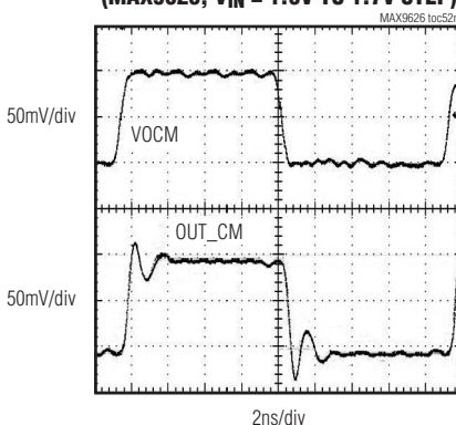
VOCM TRANSIENT RESPONSE (MAX9626, V_{IN} = 1.6V TO 1.7V STEP)
