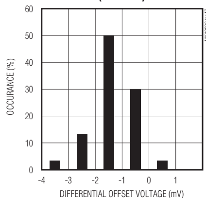
OFFSET VOLTAGE HISTOGRAM (MAX9628)
