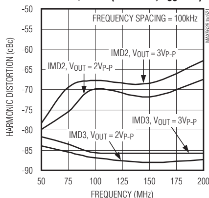
INTERMODULATION DISTORTION vs. FREQUENCY (MAX9627, V_{CC} = 5V )
