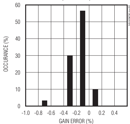
GAIN ERROR HISTOGRAM (MAX9628)
