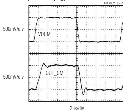
VOCM TRANSIENT RESPONSE (MAX9627, V_{IN} = 1.15V TO 2.15V STEP)
