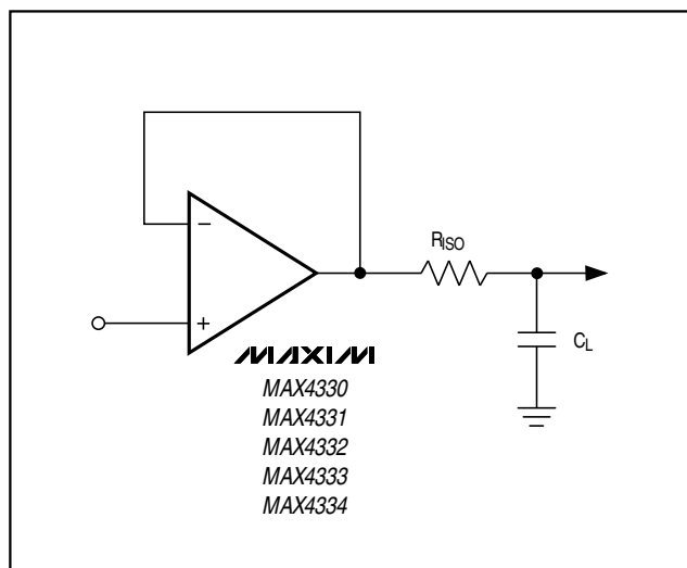
Figure 6. Capacitive-Load-Driving Circuit
