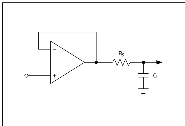
Figure 9. Capacitive-Load-Driving Circuit
