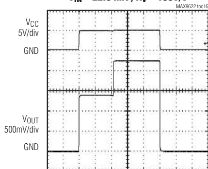
TURN-ON RESPONSE V_{IN} = 22.34mV , A_V = 100V/V
