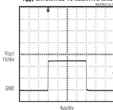
OUTPUT RECOVERY FROM SATURATION V_{OUT} SATURATED TO NEGATIVE RAIL
