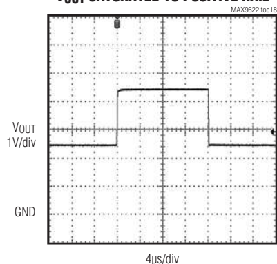
OUTPUT RECOVERY FROM SATURATION V_{OUT} SATURATED TO POSITIVE RAIL
