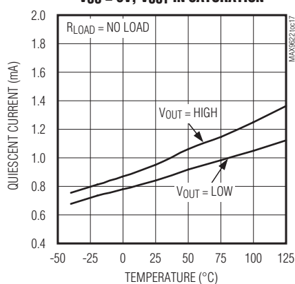
QUIESCENT CURRENT vs. TEMPERATURE V_{CC} = 5V , V_{OUT} IN SATURATION
