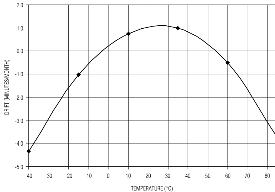
DS1922L RTC Accuracy (Typical)
