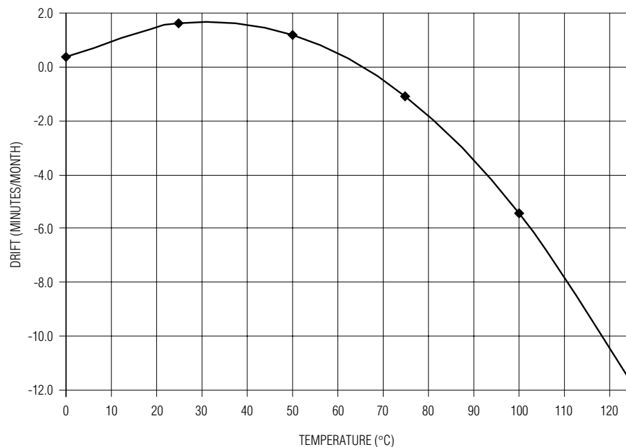
DS1922T RTC Accuracy (Typical)
