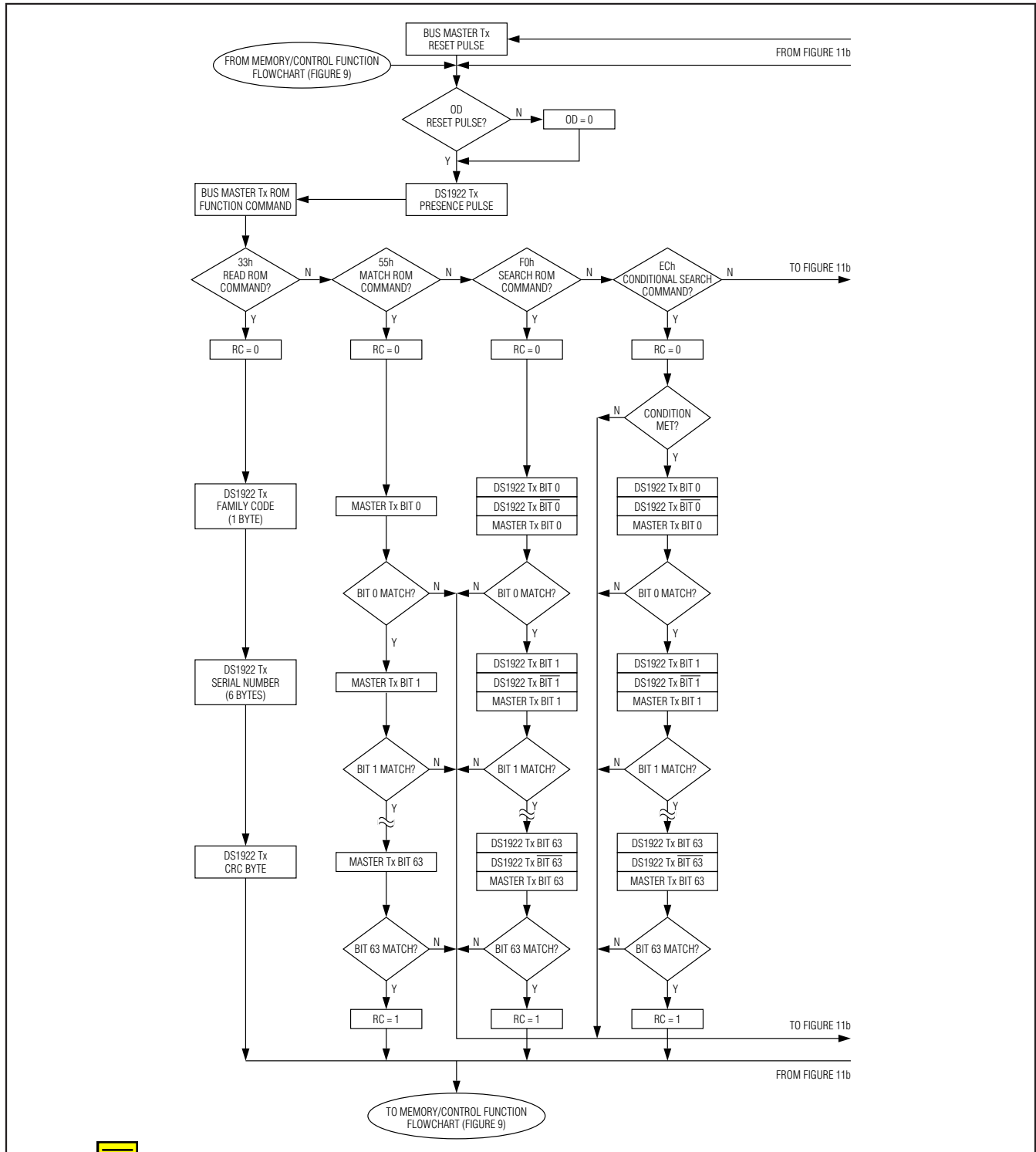
Figure 11a. Functions Flowchart
