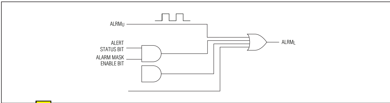
Figure 45. Diagram of Alert Conditions and Associated Alarm Enable Bits
