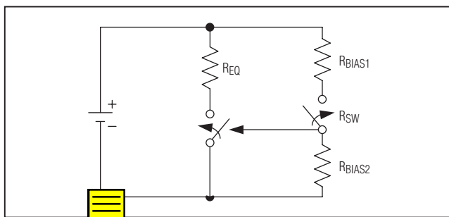
Figure 15. Simplified External Cell-Balancing Circuit
