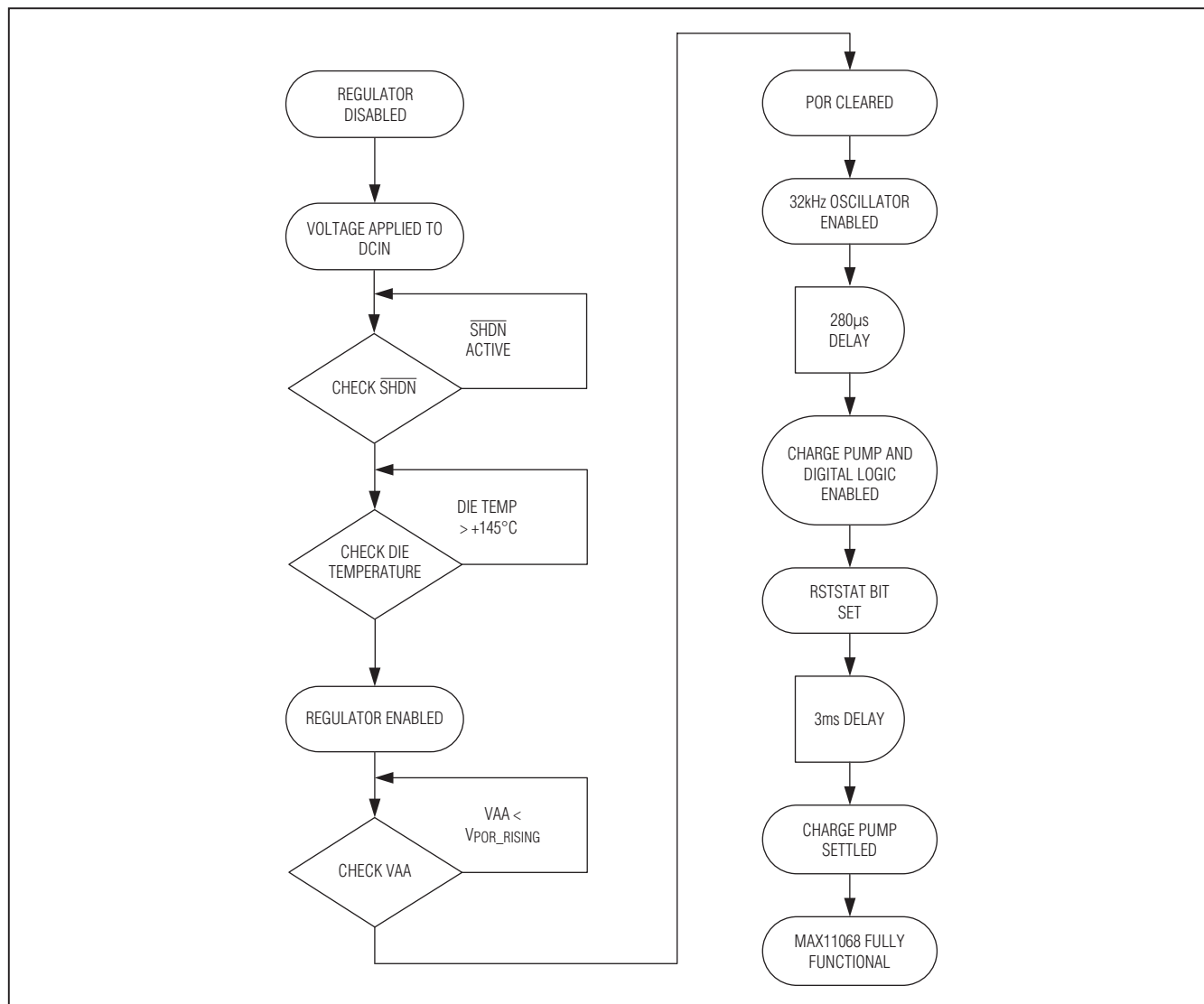
Figure 20. Power-Up Sequence
