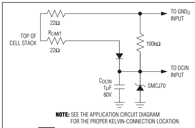
Figure 24. Overvoltage Protection and Decoupling Circuit
